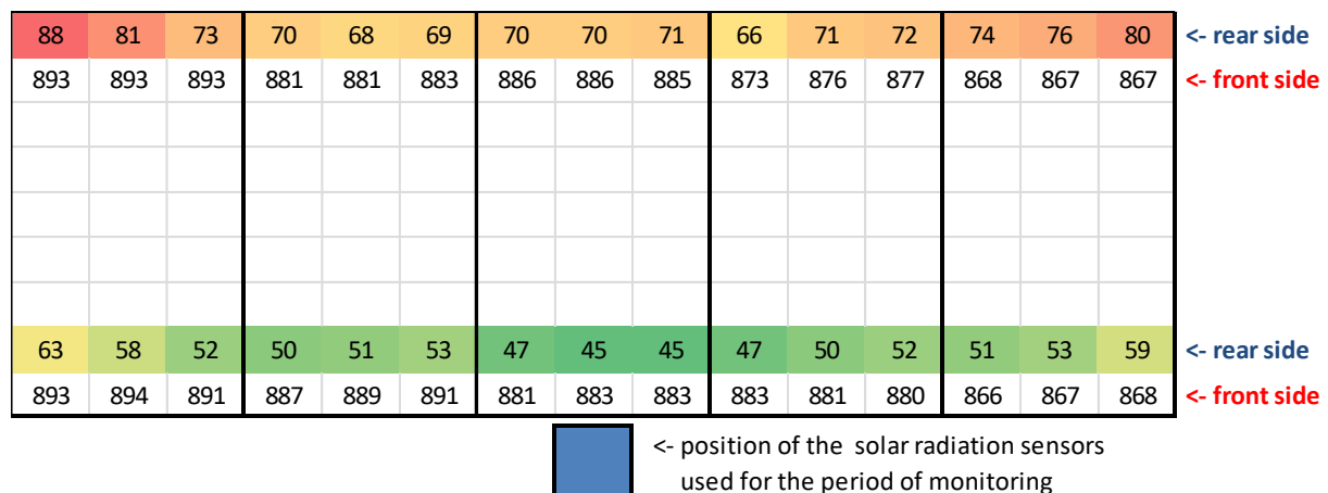
Figure 109: Measurement of the solar radiation inhomogeneity incident on the rear side of the PV modules for the test condition 3, South, 30° tilt, grass.
