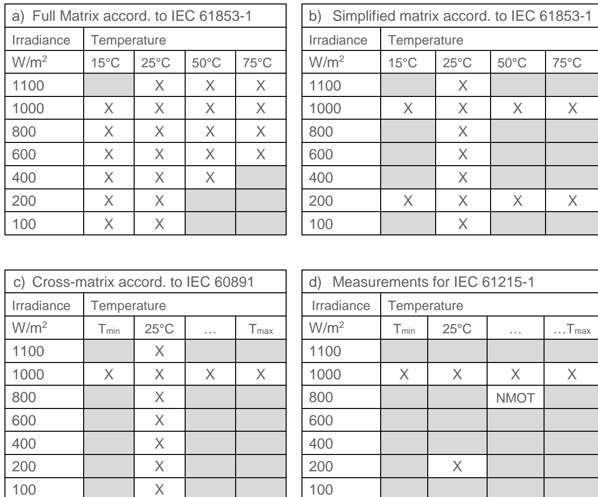
Figure 44: Different matrix configurations for module performance according to IEC testing standards.
