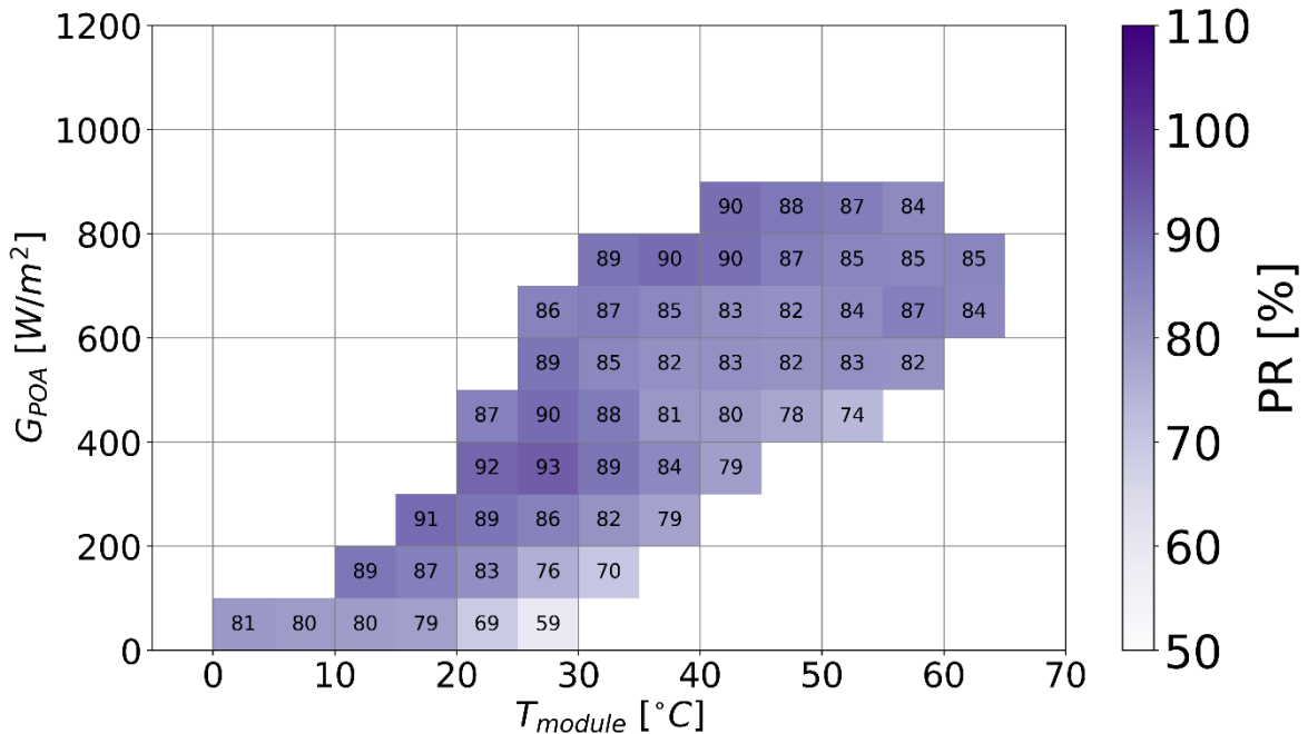
Figure 20: PR as a function of T_{mod} and G_{POA} with the fine binning. The additional threshold applied, please refer to text.
