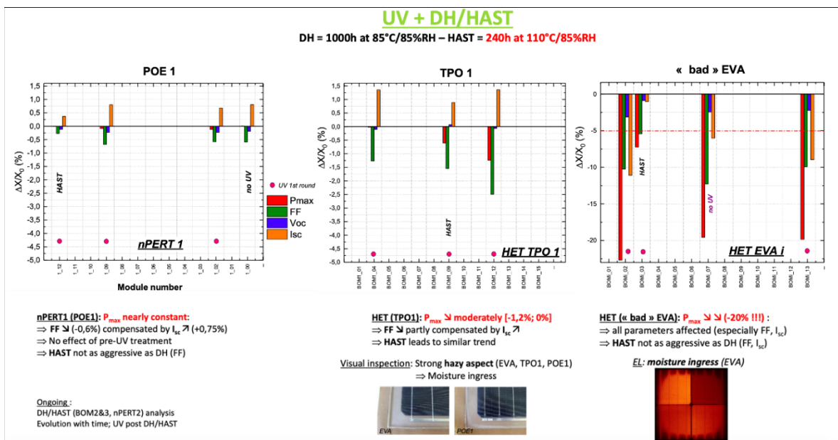
Figure 38: Assessment of heterojunction and nPERT modules with different encapsulants, following the modified indoor testing procedure (Source [109]).
