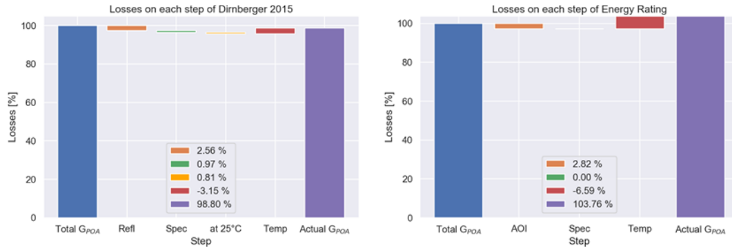
Figure 66: Relative losses to the GPOA high elevation climate. On the left, the losses from Dirnberger 2015 model. On the right side, the losses from Energy Rating model.
