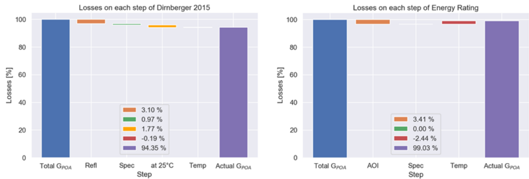
Figure 67: Relative losses to the GPOA temperate continental climate. On the left, the losses from Dirnberger 2015 model. On the right side, the losses from Energy Rating model.
