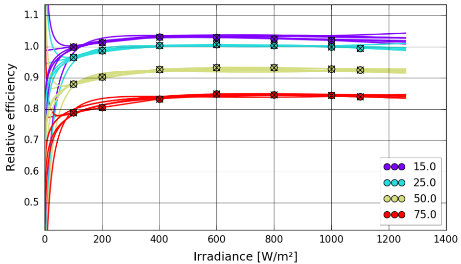
Figure 6 Superposition of all 6 models for the First Solar CdTe module showing extreme differences in extrapolation below 100 W/m²
